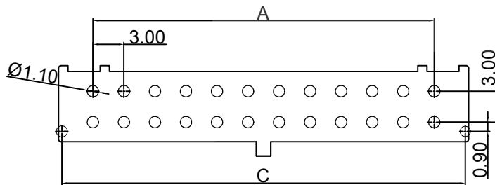
Board Layout General Tolerance: ±0.05
